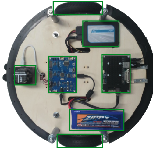
Figure 5.16: Discovery robot
