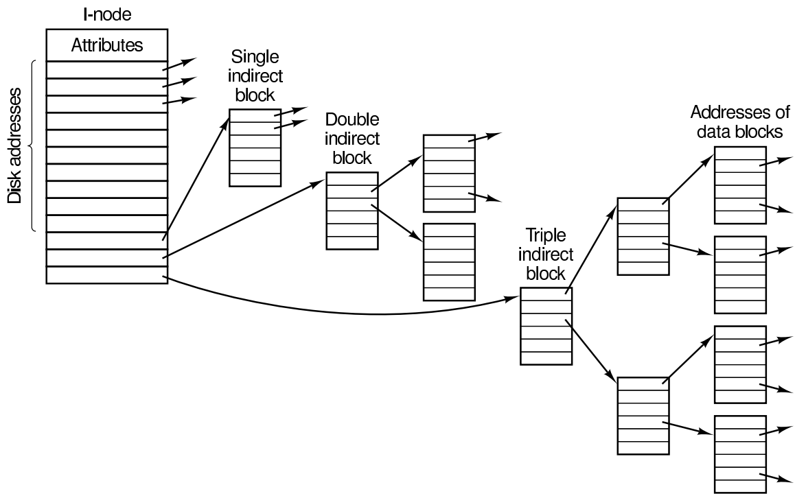
Figure 5-10. An i-node.
